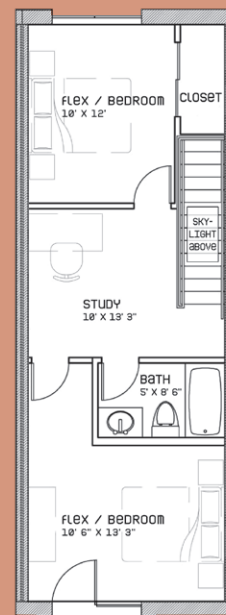
SECOND FLOOR PLAN OPTIONAL WALLS INCLUDED
