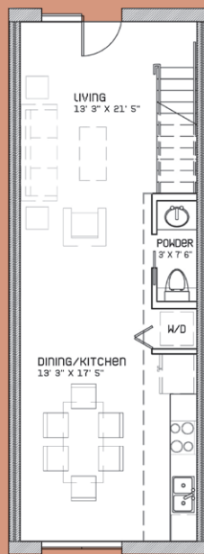
FIRST FLOOR PLAN TYPICAL FOR UNITS #10-14
